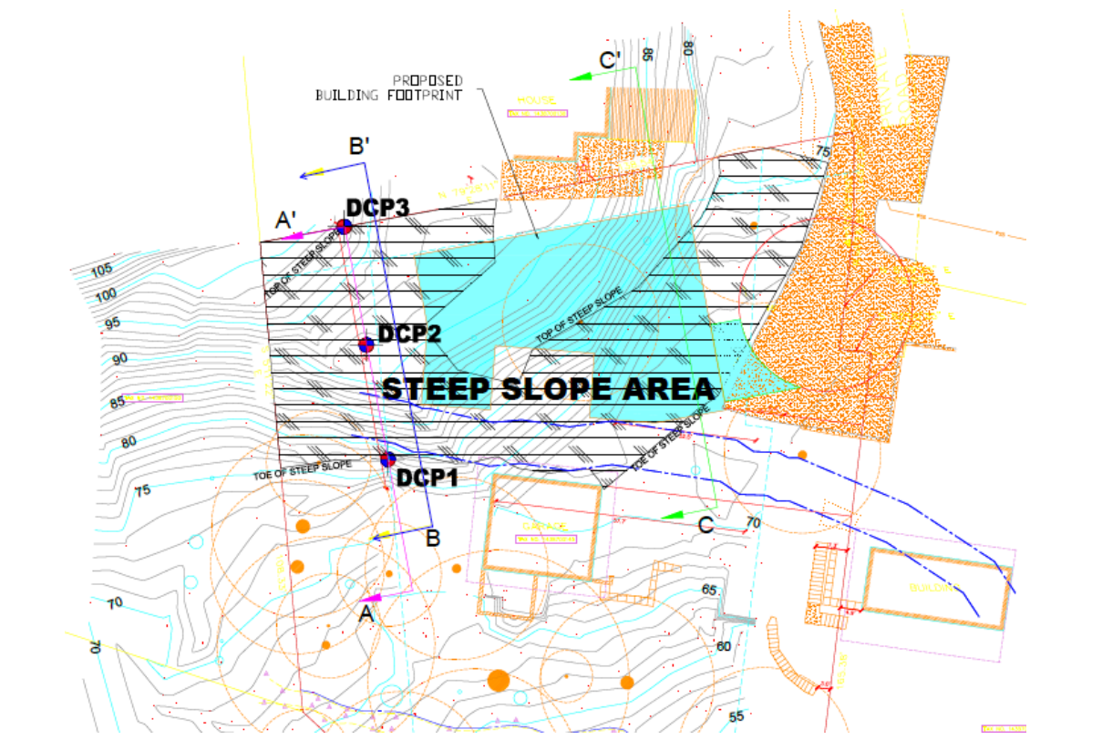
SITE PLAN
